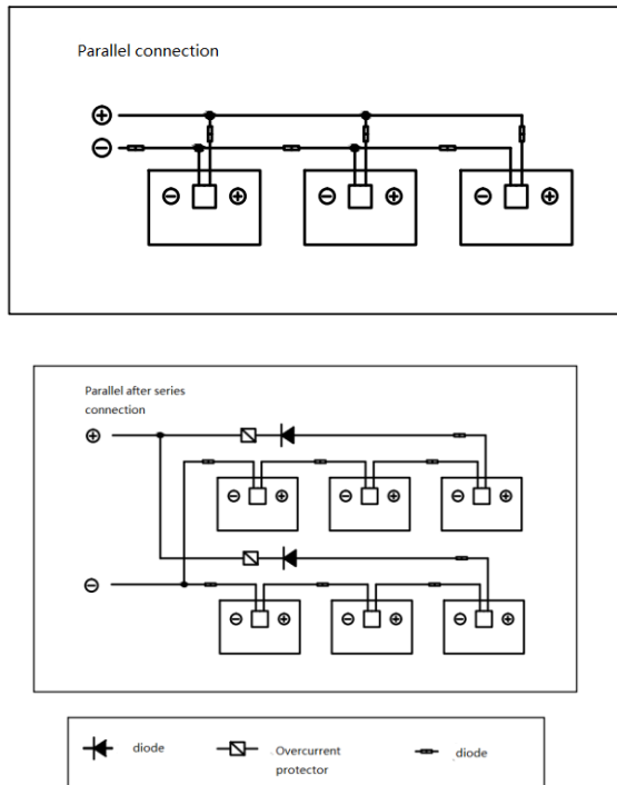
Fig. 11 Schematic diagram of electrical connection
